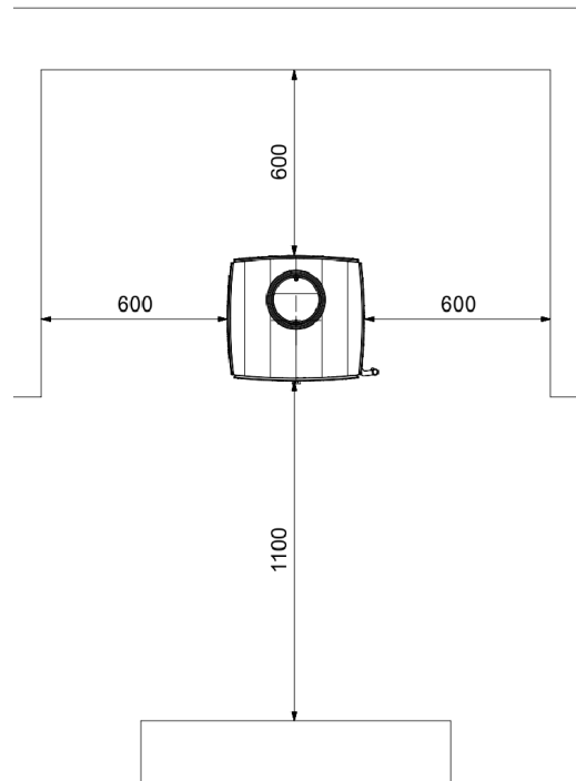
FIG. 7 SAFETY DISTANCE WITHOUT REAR PROTECTIVE PLATE (mm)
